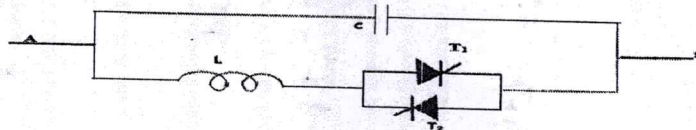
Fig.1 Circuit diagram of TCSC
