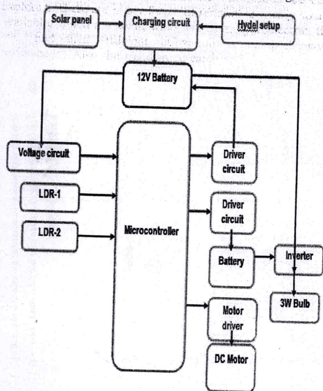
Fig.1: Block Diagram
